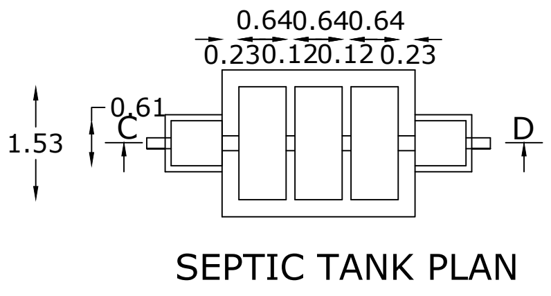
SEPTIC TANK PLAN ALL DIMENSION ARE IN METRE SCALE 1:100
