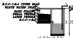
RECYCLING OF WASTE WATER KITCHEN & BATH ROOM
