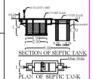
RECYCLING OF WASTE WATER KITCHEN & BATH ROOM
