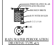
RAIN WATER PERCOLATION DRAWING TYPE -1A
