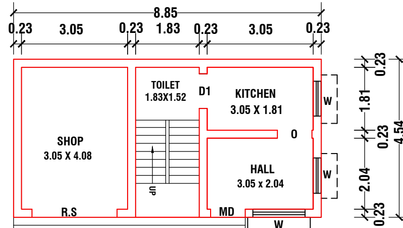
GROUND FLOOR PLAN SCALE 1:100 ALL DIMENSIONS ARE IN METER
