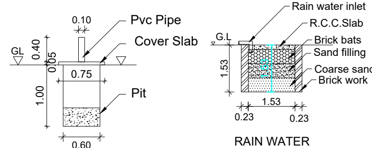
RAIN WATER HARVESTING PIT
