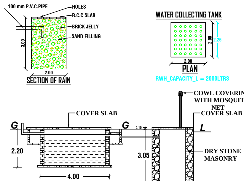
SEPTIC TANK WITH SOAK PIT
