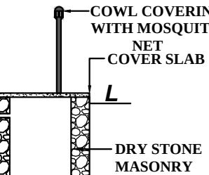
SEPTIC TANK WITH SOAK PIT
