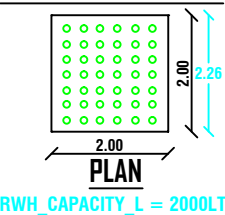
WATER COLLECTING TANK
