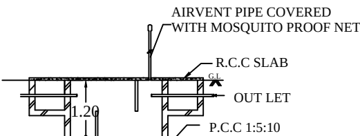
L.S. OF SEPTIC TANK
