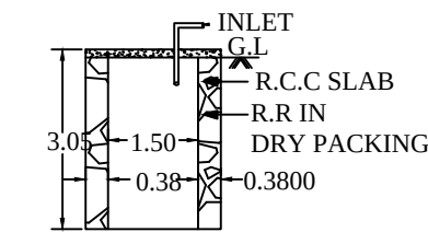
RAIN WATER HARVESTING
