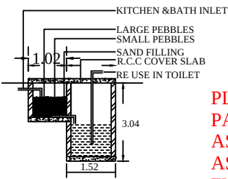
DETAILS OF RECYCLING OF WASTE
