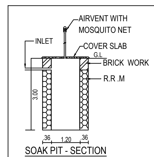
SOAK PIT - SECTION
