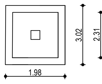
COMPOST PIT - PLAN
