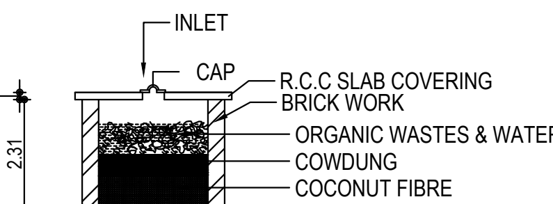
COMPOST PIT - SECTION
