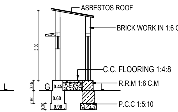
SECTION ON - JK
