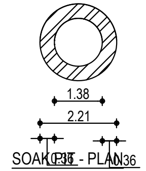
SOAK PIT - PLAN
