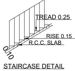
STAIRCASE DETAIL
