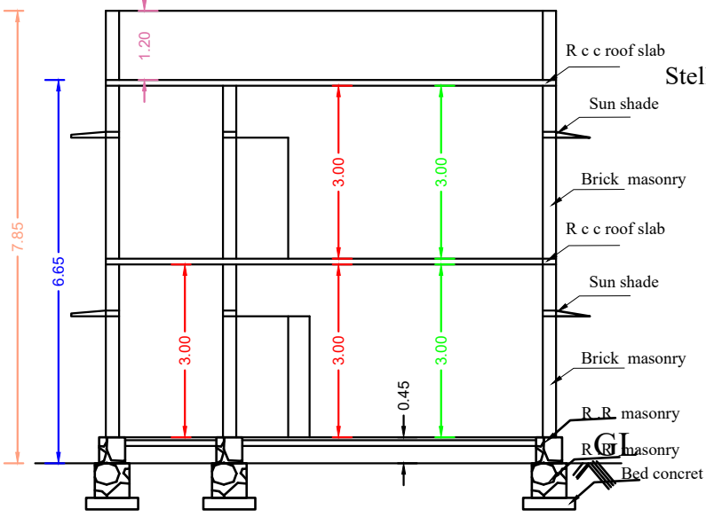
SECTION ON GG
