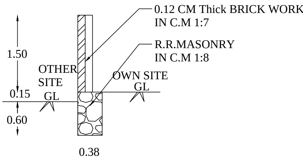
SECTION ON 'CD'
