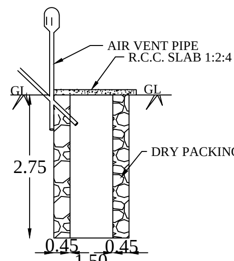
SOAK PIT DETAILS
