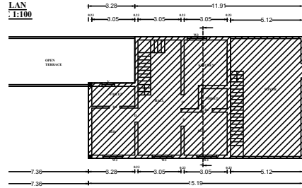
EXISTING FIRST FLOOR PLAN
