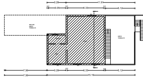
EXISTING SECOND FLOOR PLAN
