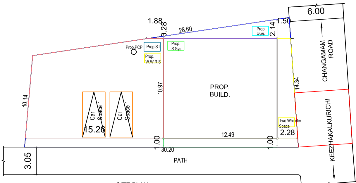
SITE PLAN SCALE:1:200
