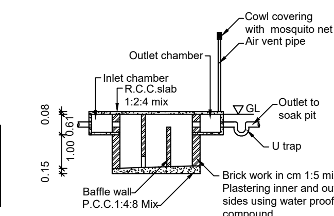
SECTION UV
