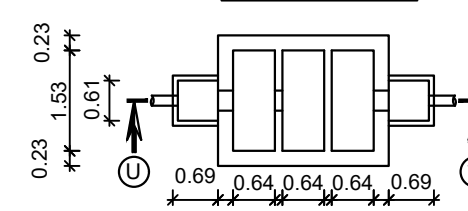
SECTION UV
