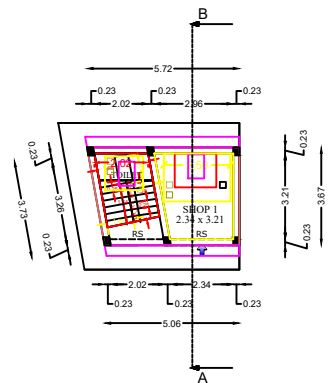
GROUND FLOOR PLAN (scale 1:100 )
