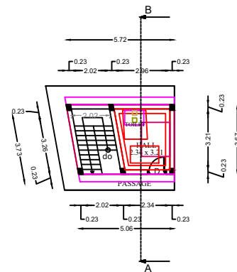
FIRST FLOOR PLAN (scale 1:100 )
