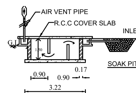
SEPTIC TANK
