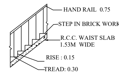
STAIR CASE SECTION
