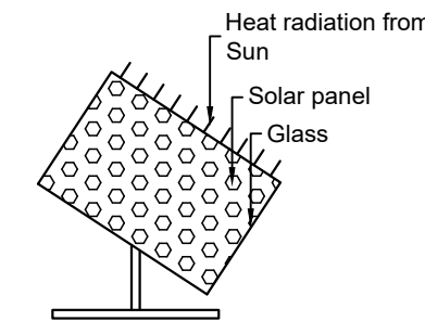
SOLAR SYSTEM
