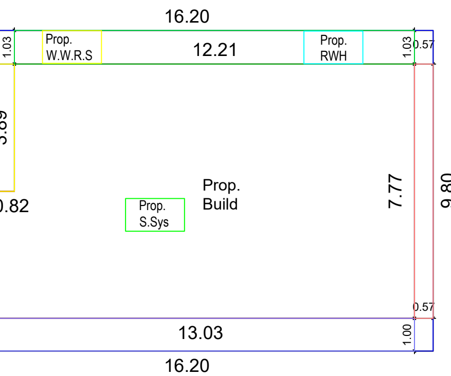
SOLAR SYSTEM
