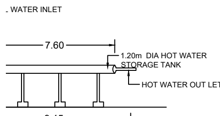
SOLAR WATER HEATING SYSTEM(S.W.H.S. DETAILS)
