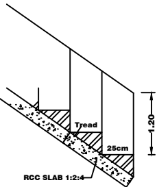
STAIR DETAILS
