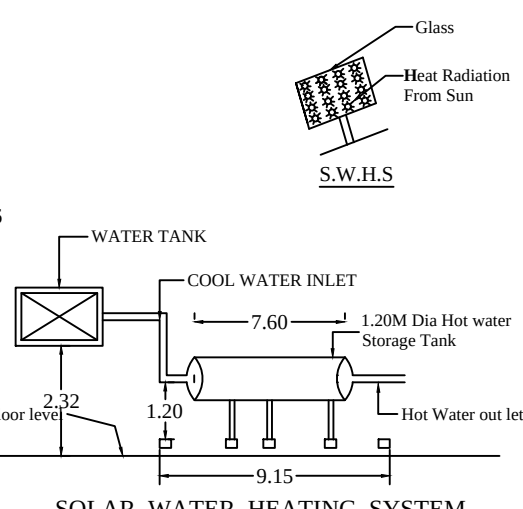
SOLAR WATER HEATING SYSTEM (S.W.H.S.DETAILS)
