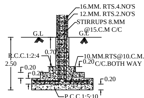
COLUMN SECTION
