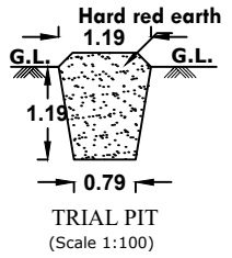
TRIAL PIT (Scale 1:100)
