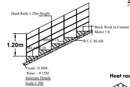
Hand Rails-1.20m Height
