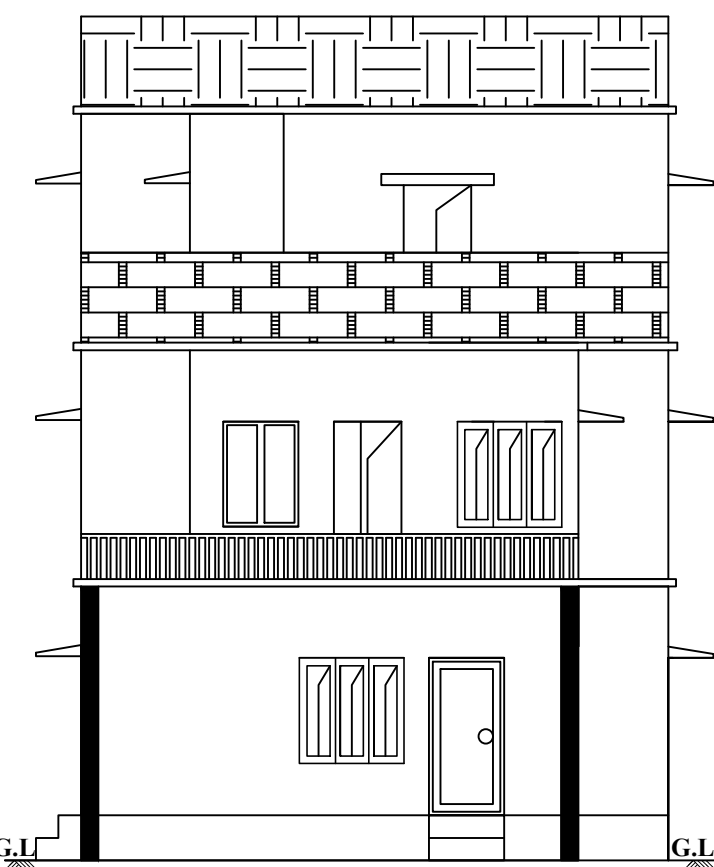
FRONT ELEVATION
