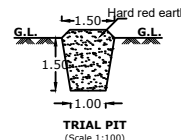
TRIAL PIT
