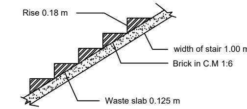
Stair Details
