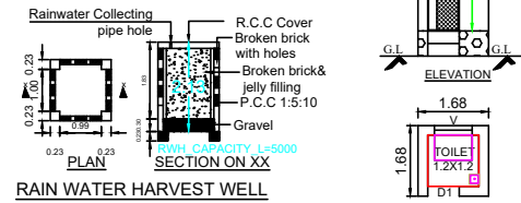
RAIN WATER HARVEST WELL
