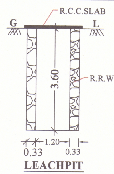
LEACH PIT
