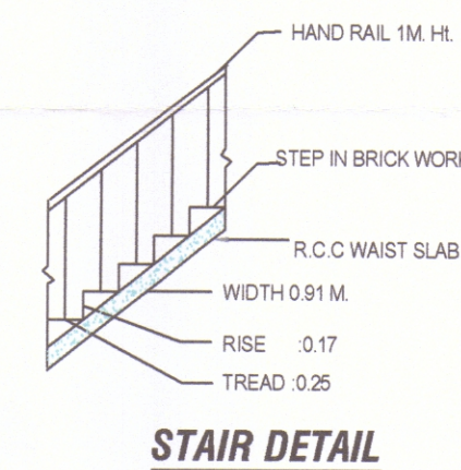
STAIR DETAIL
