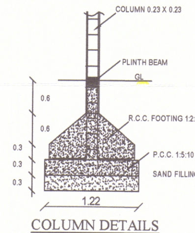
COLUMN DETAILS
