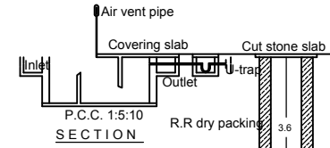
TRAIL PIT NOT TO SCALE
