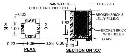
RAIN WATER HARVEST WELL
