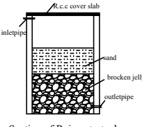
Section of Rainwatertank
