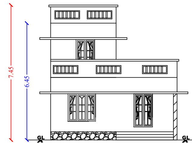
ELEVATION SCALE 1:100
