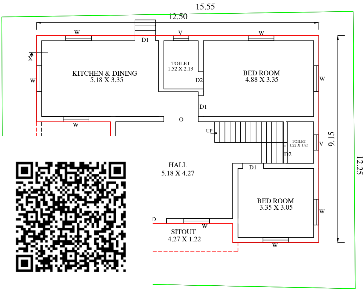
SITE CUM GROUND FLOOR PLAN
