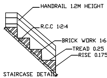
STAIRCASE DETAILS
