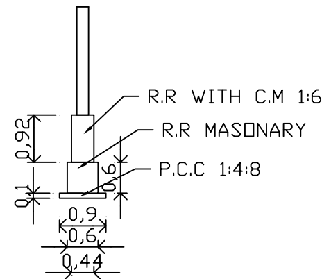
FOUNDATION
