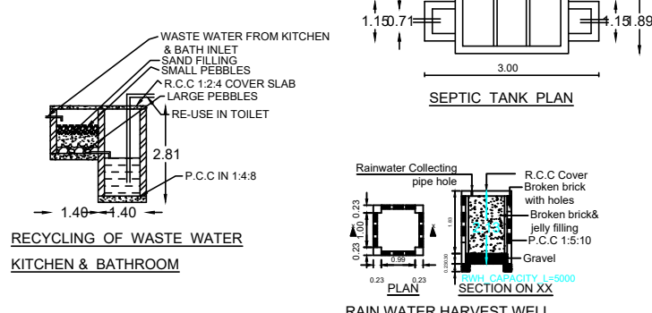
RAIN WATER HARVEST WELL
