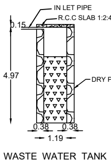
WASTE WATER TANK
