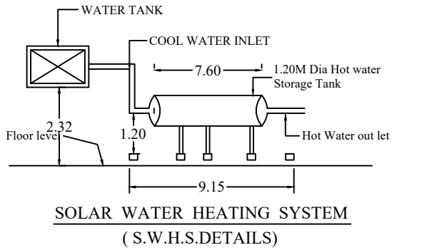
SOLAR WATER HEATING SYSTEM (S.W.H.S.DETAILS)
