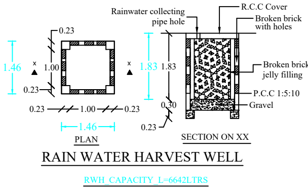
RAIN WATER HARVEST WELL RWH CAPACITY 1=6642LTRS
