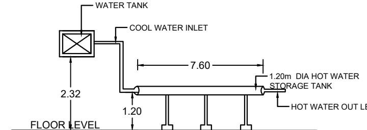
SOLAR WATER HEATING SYSTEM(S.W.H.S. DETAILS)
