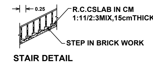
STAIR DETAIL
