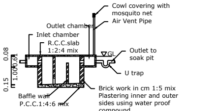
SECTION UV
