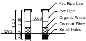
PIPE COMPOST PIT
