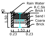
RAIN WATER HARVESTING PIT
