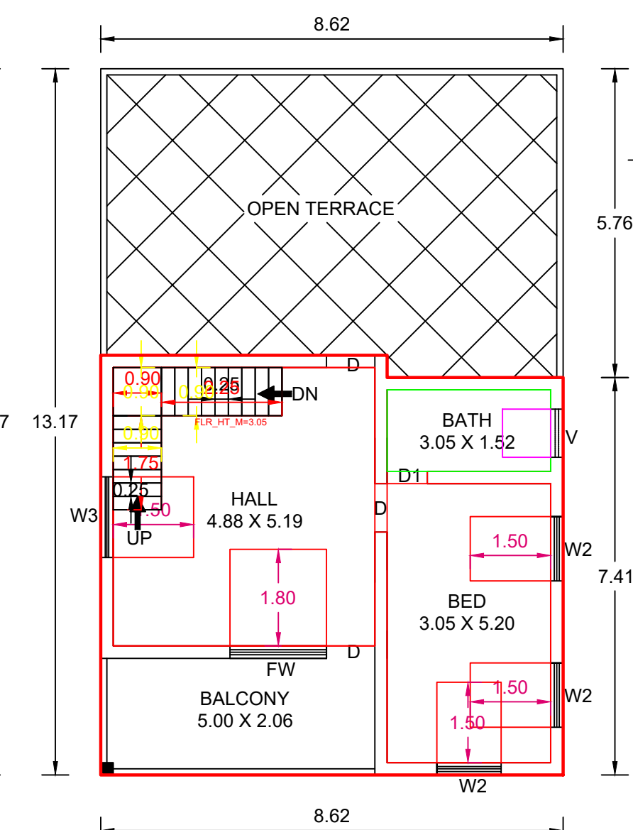
FIRST FOOR PLAN
