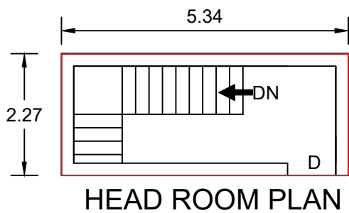
HEAD ROOM PLAN
