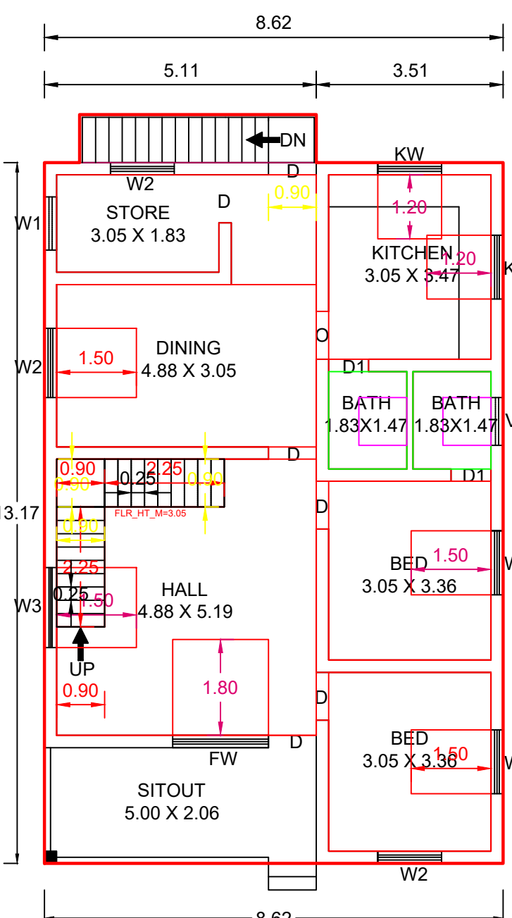
GROUND FOOR PLAN
