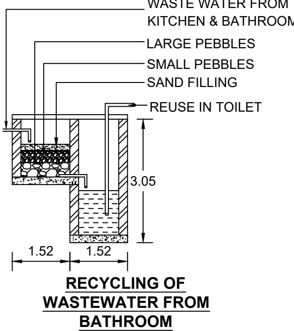
RECYCLING OF WASTEWATER FROM BATHROOM
