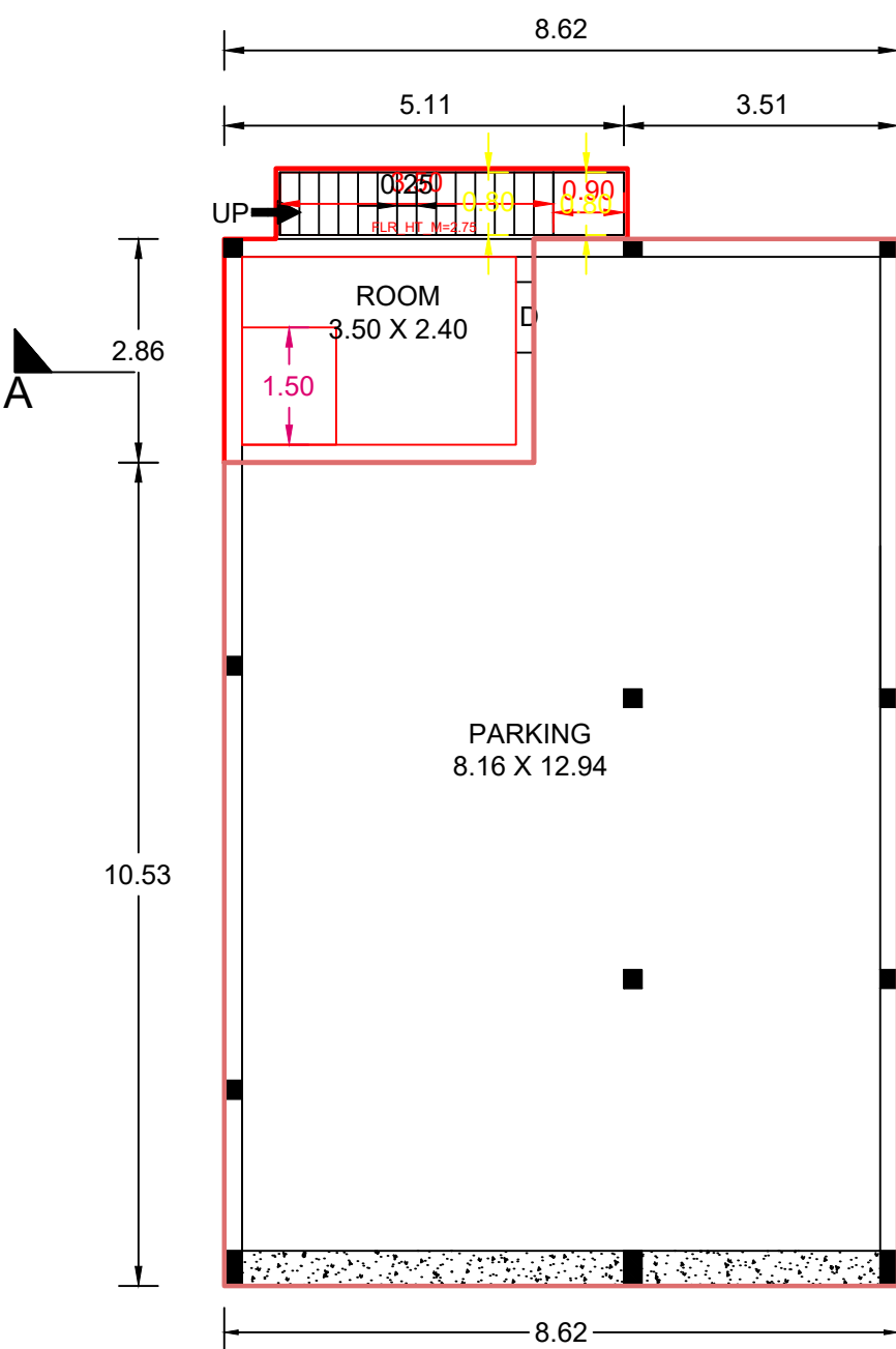
STILT FOOR PLAN
