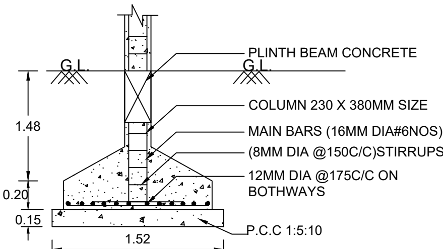
COLUMN FOOTING
