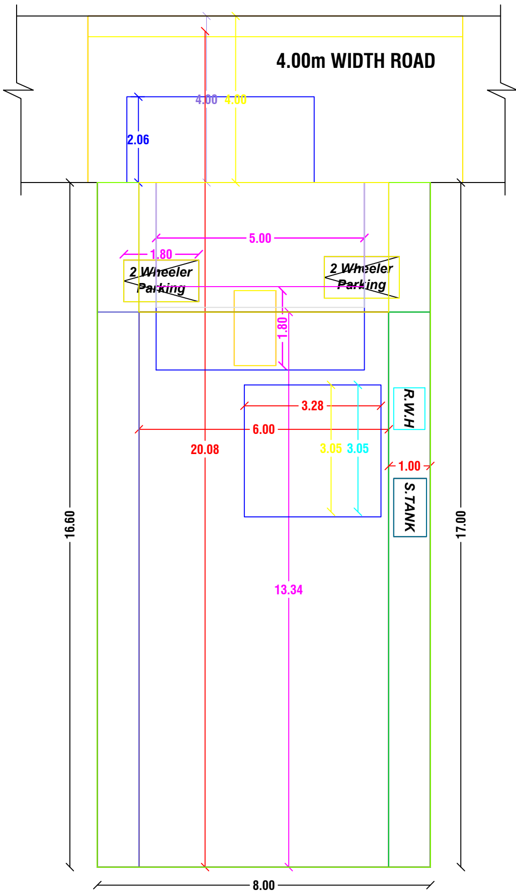
SITE PLAN
