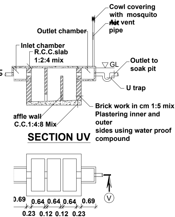
SEPTIC TANK PLAN
