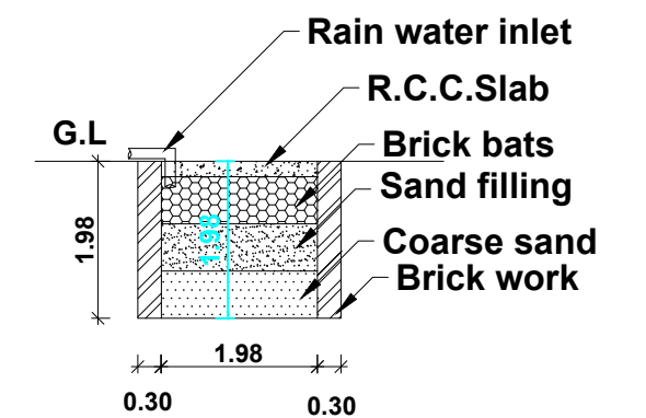
RAIN WATER HARVESTING PIT
