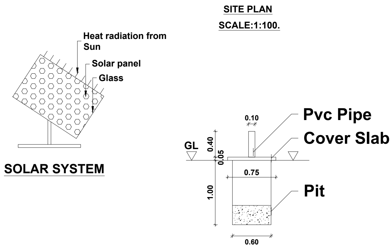
SOLID WASTE COMPOST PIT
