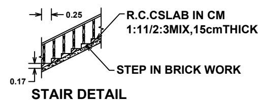
STAIR DETAIL
