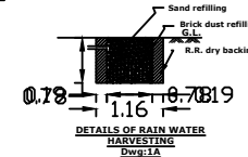
DETAILS OF RAIN WATER HARVESTING Dwg: 1A
