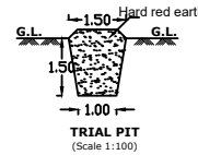
TRIAL PIT (Scale 1:100)
