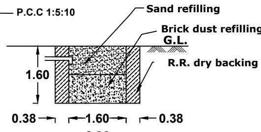
DETAILS OF RAIN WATER
