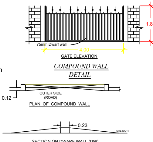
SECTION ON DWARF WALL (DW) (NOT TO SCALE)
