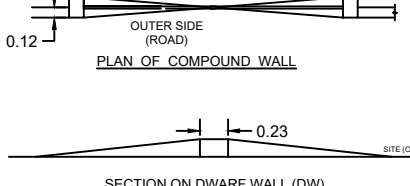
SECTION ON DWARF WALL (DW) (NOT TO SCALE)
