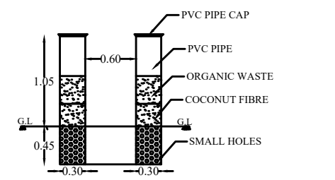
PIPE COMPOSIT PIT
