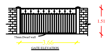
GATE ELEVATION
