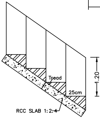
STAIR DETAILS
