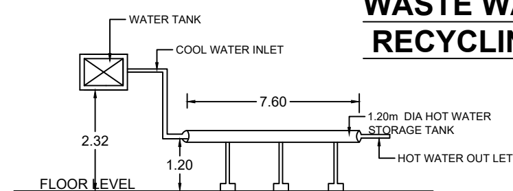
SOLAR WATER HEATING SYSTEM(S.W.H.S. DETAILS)
