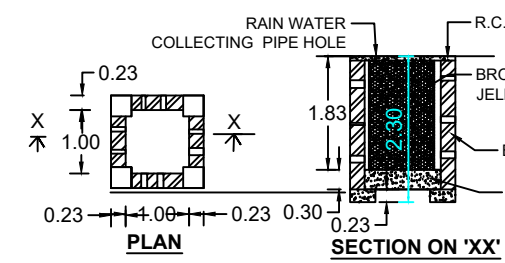
RAIN WATER HARVEST WELL
