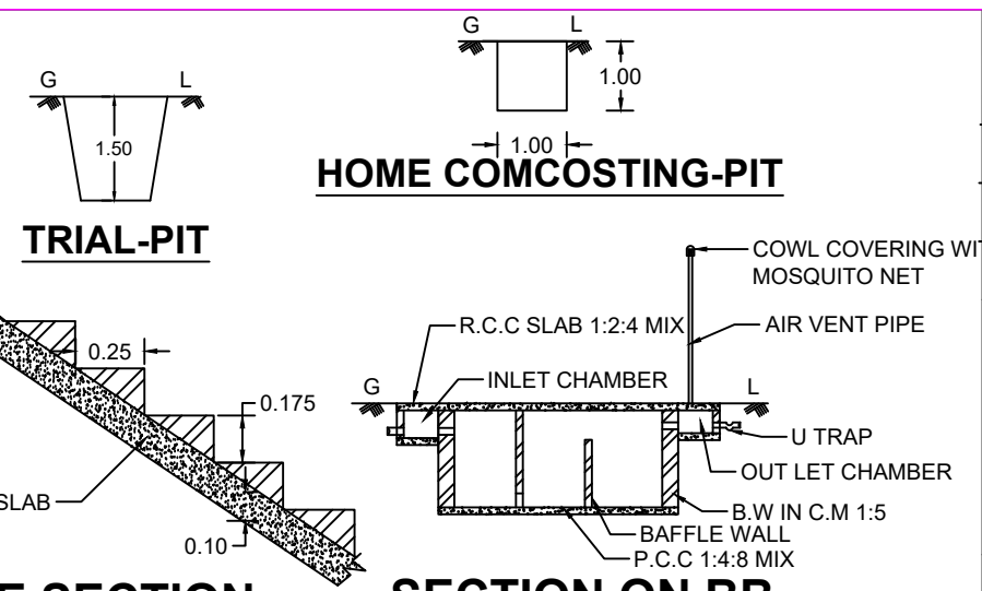
STAIR CASE SECTION
