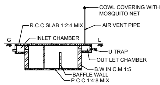
SECTION ON BB
