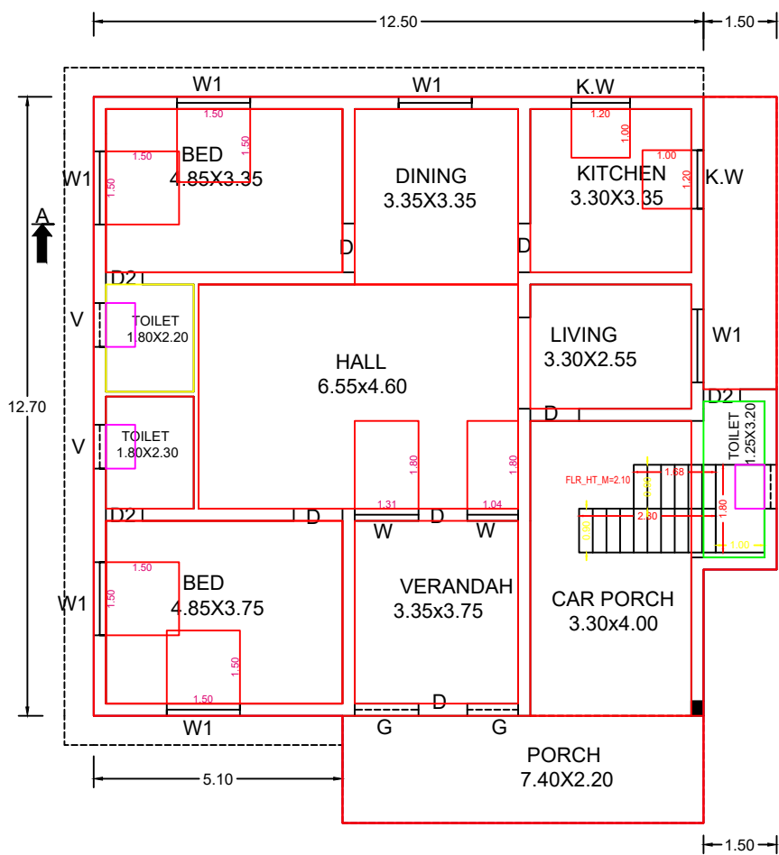
G.F. PLAN
