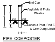
PIPE COMPOSTER
