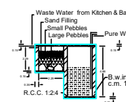
WASTE WATER RECYCLING SYSTEM
