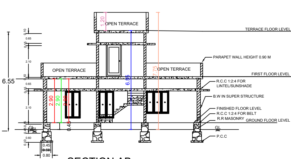
SECTION AB
