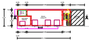
PLAN OF GROUND FLOOR
