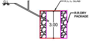
SECTION OF SOAKPIT
